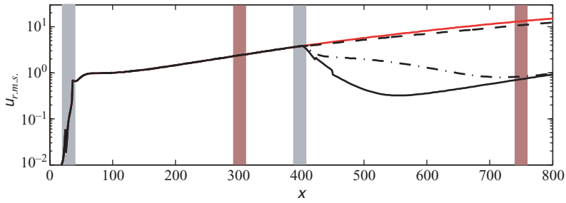
FIGURE 15. The r.m.s. values of the uncontrolled system (red line), cheap controller (solid black), intermediate controller (dashed–dotted line) and expensive controller (dashed line). The grey bars represent the size (defined as 99% of the spatial support) and the location of the two inputs, whereas the red bars correspond to the two outputs.
